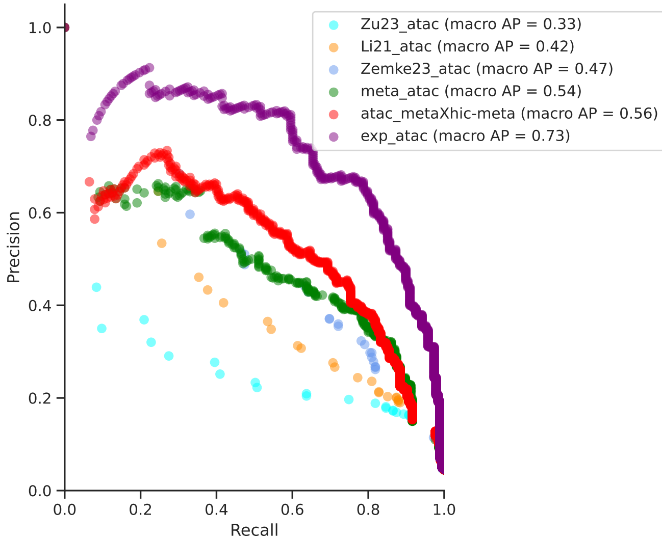
Summary Precision-Recall Curve
