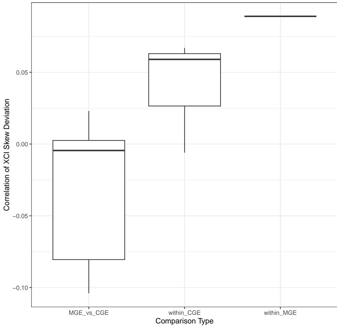
Boxplot of Correlations
