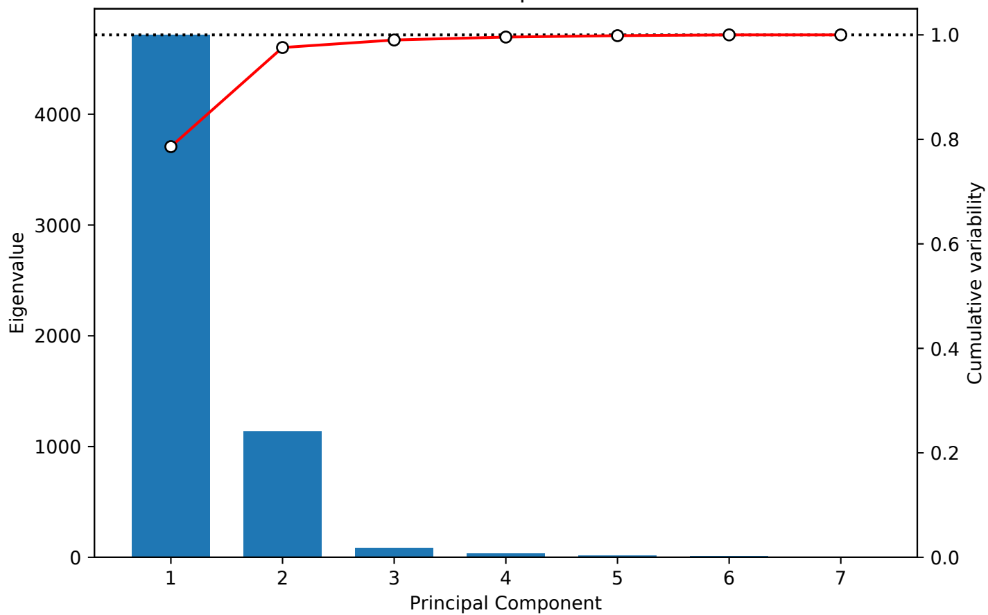
Scree plot
